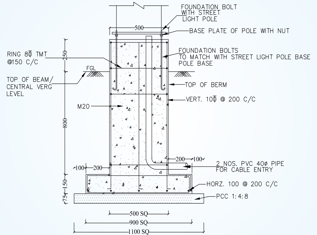
FOUNDATION DETAILS FOR 10/12M HIGH OCTAGONAL POLE
